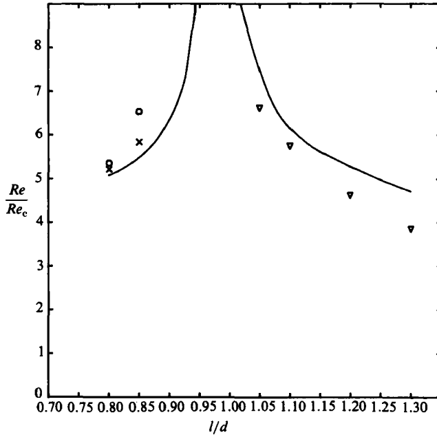
FIGURE 6. Neutral stability curves for m = 1 at \eta = 0.56 , in the (Re/Re_c, l/d) -plane: —, best fit through Cole's data; ▽, computed points for the classical wavy mode; ○, computed points for the harmonic jet mode; ×, computed points for the subharmonic jet mode. Points with l/d less than 1 refer to the jet modes: points with l/d greater than 1 refer to the usual wavy mode.
