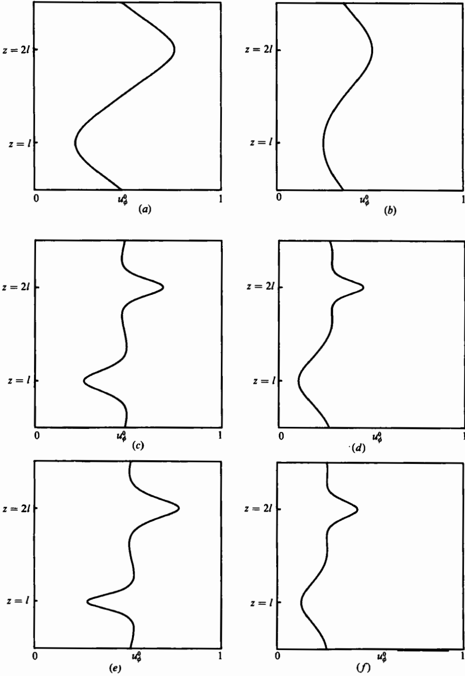
FIGURE 11. Velocity profiles u_0^0(z) at r = \frac{1}{2}(R_1 + R_2) . The parameter values correspond to those in figure 10.
